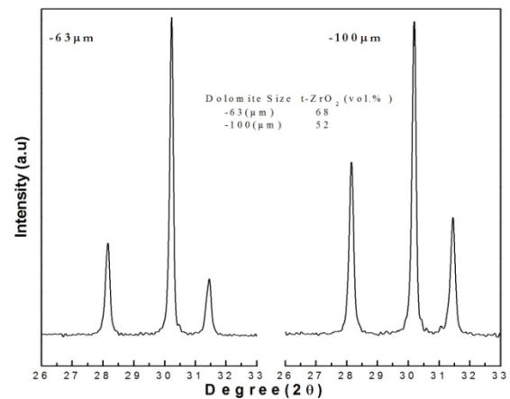
Figure 1. X-ray diffraction pattern of calcined zirconia-6mole% dolomite powder
