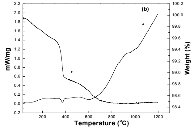
Figure 2. (a) DSC/TG behavior of dolomite and (b) DSC/TG behavior of zirconia-6mole% dolomite powder
