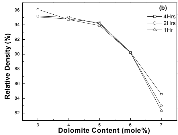
Figure 5. Relative density of dolomite-ZrO 2 as a function of dolomite content (a) at 1550°C, (b) at 1600°C
