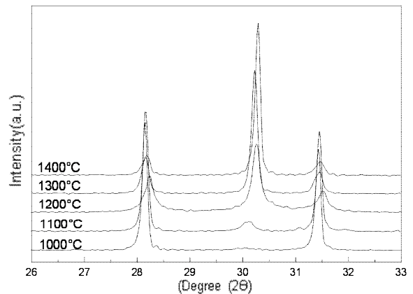
Figure 3. XRD pattern of the calcined zirconia-6 mol% dolomite composition as function of temperature
