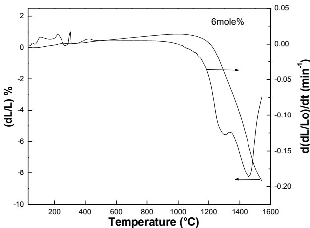
Figure 4. Non-isothermal densification behavior of zirconia-6 mole% dolomite powder
