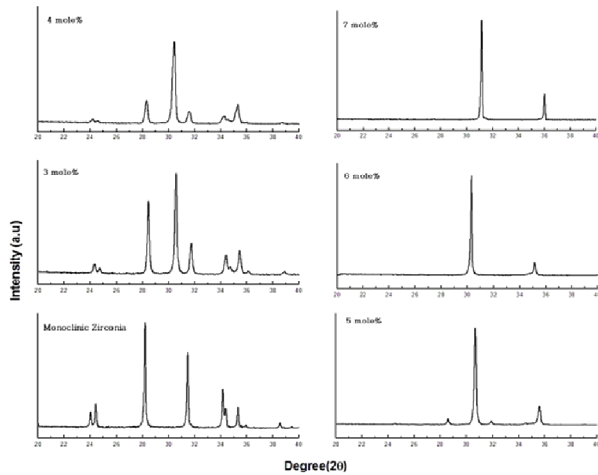
Figure 5. (c) Phase analysis of dolomite-ZrO 2 sample fired at 1600°C
